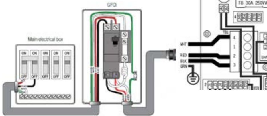
240 VOLT 60 HZ SINGLE PHASE GFCI WIRING
